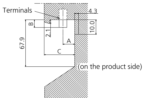
Sectional view of terminal a (VIDEO IN / PC IN / DVI-D IN)
