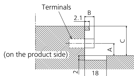
Sectional view of terminal b (USB/LAN/SERIAL)
