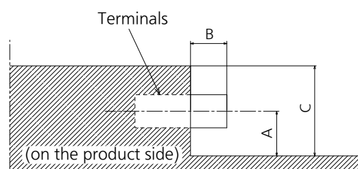
Sectional view of terminal b (USB/LAN/SERIAL)
