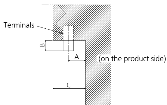
Sectional view of terminal a (VIDEO IN / PC IN / HDMI / DVI-D IN)
