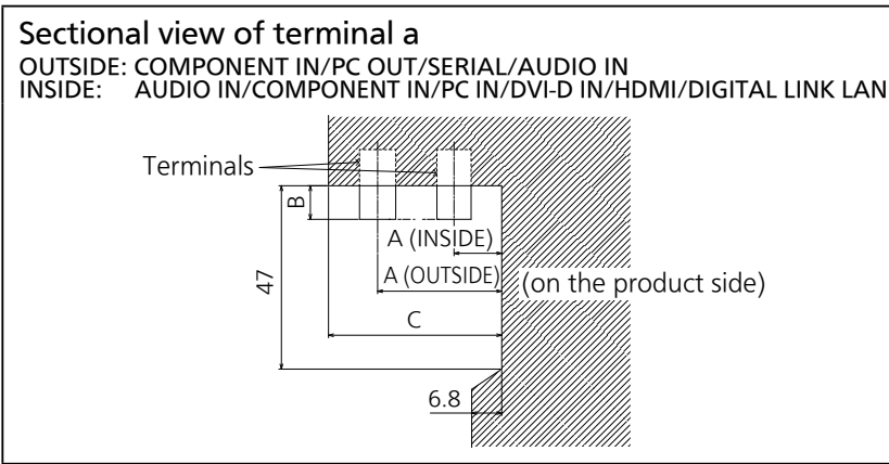
Terminal a 50BF1 Terminal (Bottom)
