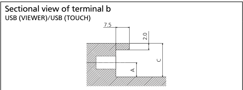
Terminal b 50BF1 Terminal (Side)
